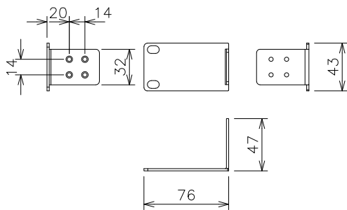
Mounting bracket (for 19-inch rack)
